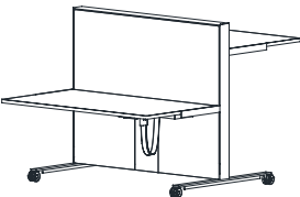
Electrified Z desk workstation with 2 height-adjustable table tops supported by castors 148x175xH126 cm
