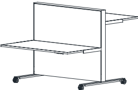
Z desk workstation with 2 height-adjustable table tops supported by castors 148x175xH126 cm
