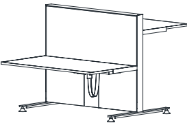
Electrified Z desk workstation with 2 height-adjustable table tops supported by feet 148x175xH124 cm
