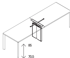
Height-adjustable center leg/cable riser for aligned workstations
