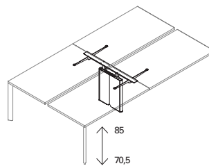
Height-adjustable center leg/cable riser for double workstations
